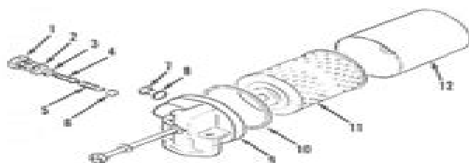
Fig. S2-1—Exploded view of engine oil filter assembly and oil pressure relief valve.
