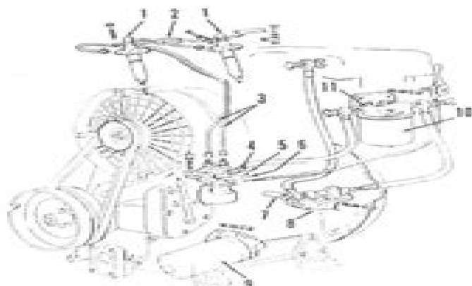
Fig. S2-2—View of fuel system components. Pump mounting gasket (10) is used to adjust injection timing.
