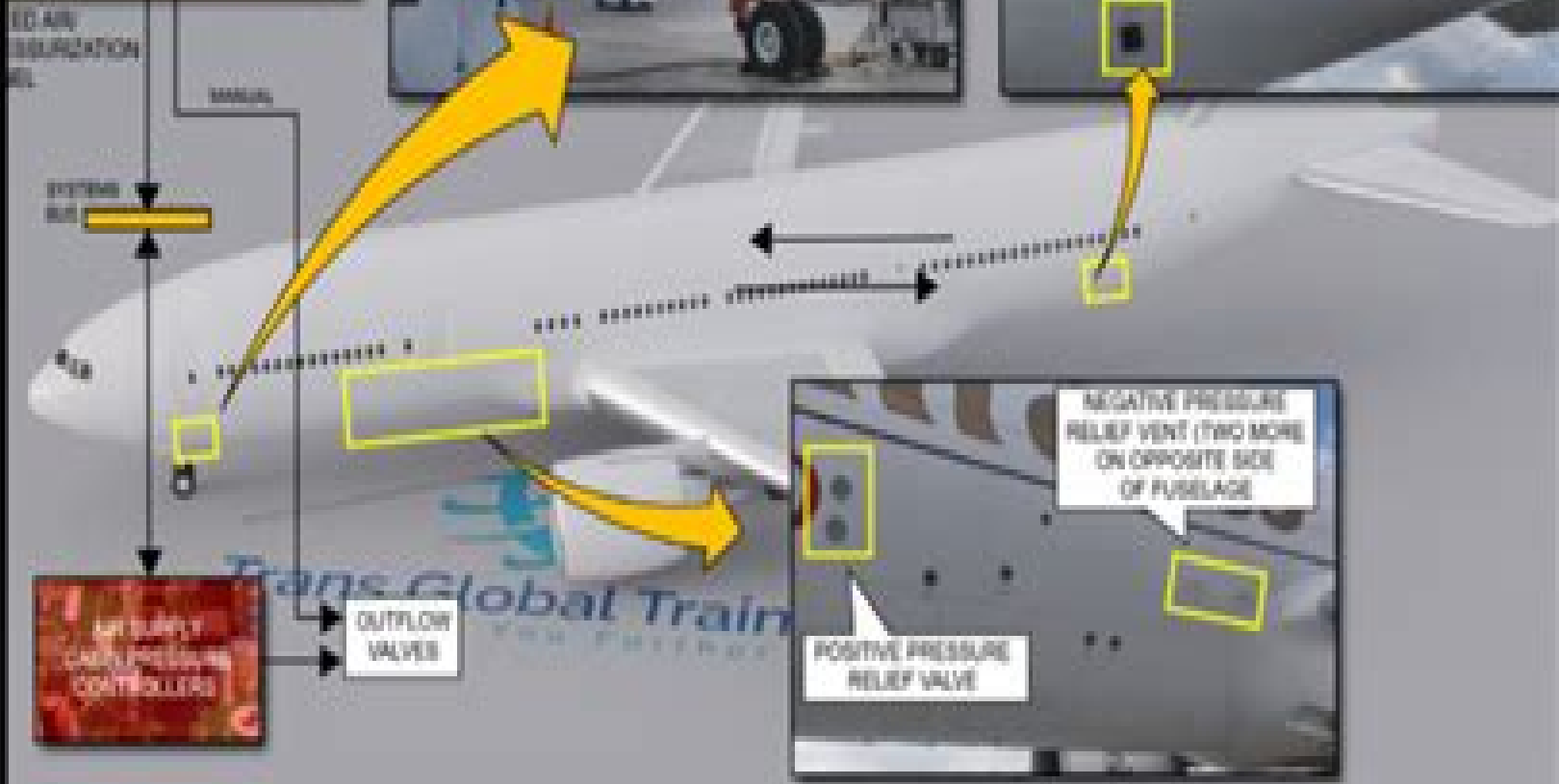
AIR CONDITIONING - PRESSURISATION
