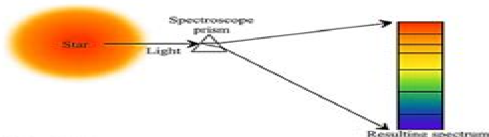
Figure 1. Spectroscopy.
