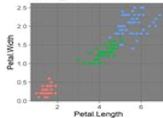
theme_dark()
