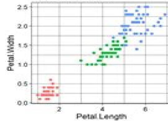
theme_linedraw()
