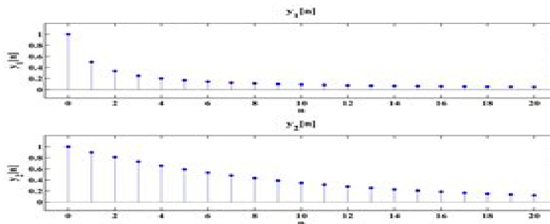
FIGURE 2.12: System responses with respect to input signal x[n] = \delta[n] .
