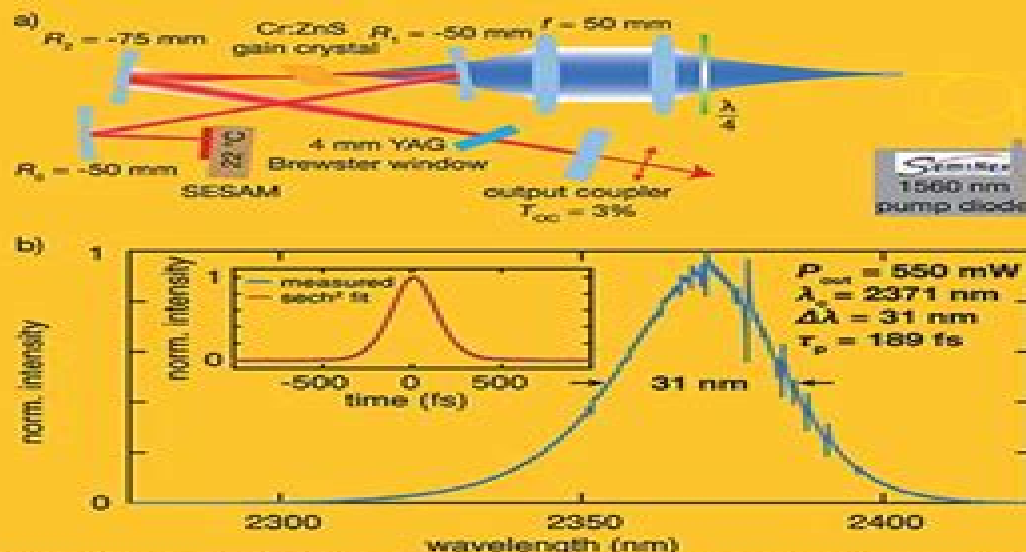
(a) X-fold standing-wave cavity for modelocked Cr:ZnS oscillator. (b) Output spectrum and intensity autocorrelation measurement (IAC). See "Low-Noise Femtosecond SESAM Modelocked Diode-Pumped Cr:ZnS Oscillator," U. Holdrich et al., Article #1300107.
