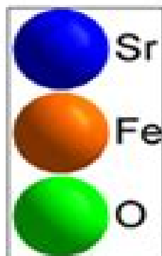
Fe512k-octahedral 4+
