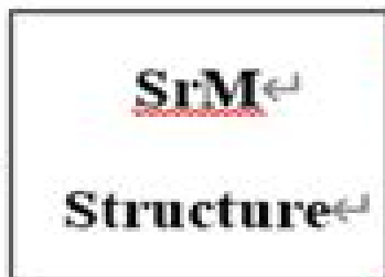
Fe3-4f 1 -tetrahedral 4+
