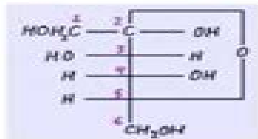
α-D (-) fructofuranose
