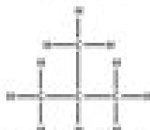
2-METHYL PROpane
