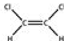
(Z)-1,2-DICHLOROETHENE Z = same side
