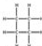
CYCLOBUTANE
