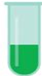
BROMOTHYMOLO BLUE
