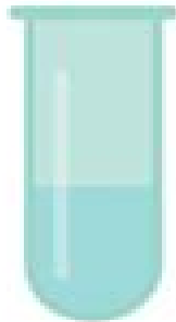
PHENOLPHTHALEIN
