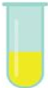
METHYL ORANGE
