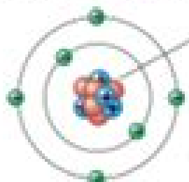
Carbon atom
