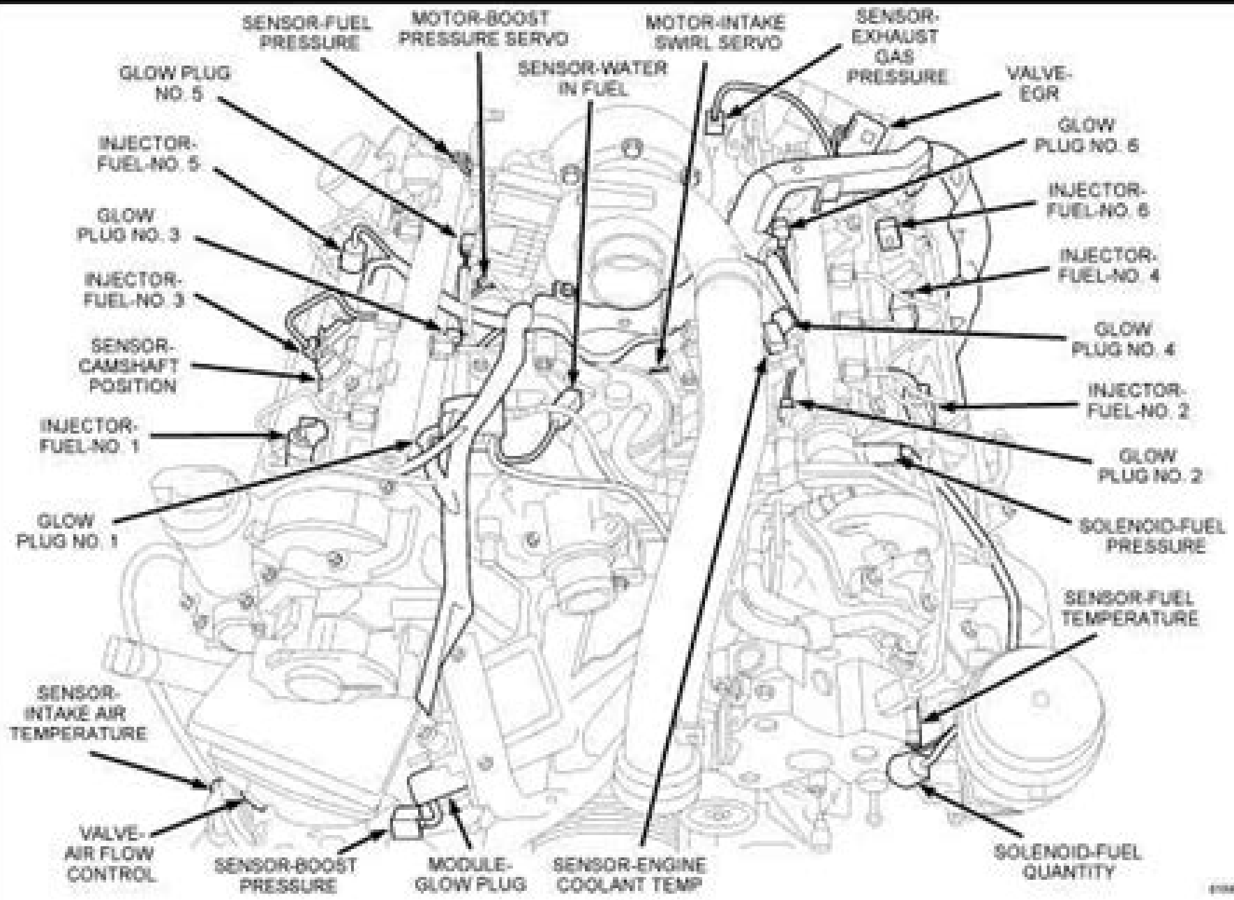
ENGINE (3.0L)
