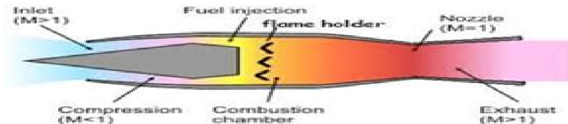
Figure 4.5 ramjet
