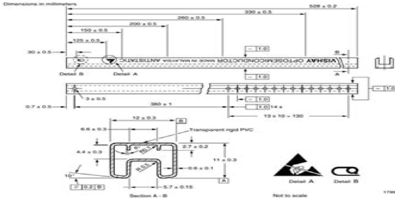
Fig. 1 - Shipping Tube Specifications for DIP Packages
