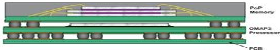
Figure 1. OMAP35x Processor (bottom device) and PoP Memory (top device) Stack Up on PCB
