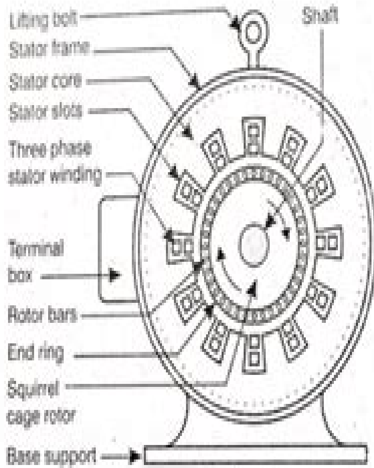
Sectional view
