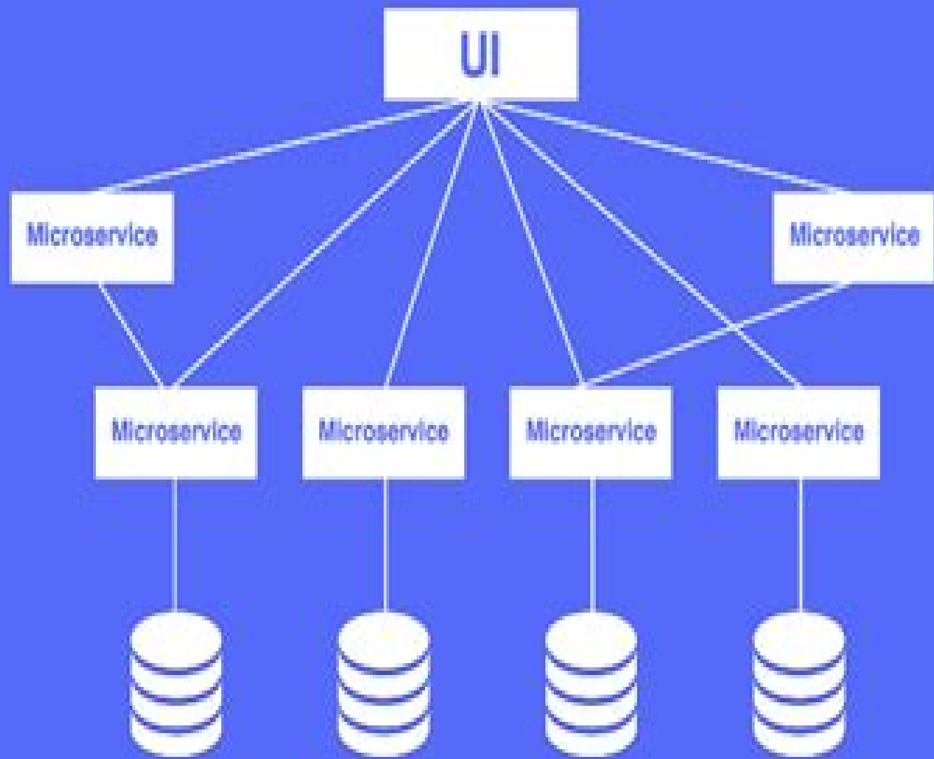
Microservices Architecture
