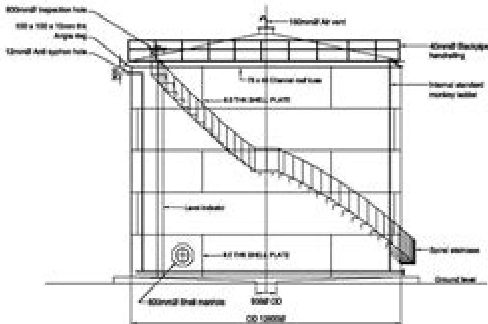
FRONT ELEVATION
