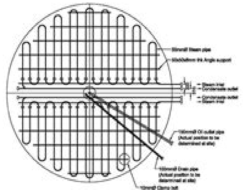
ARRANGEMENT OF STEAM HEATING PIPE
