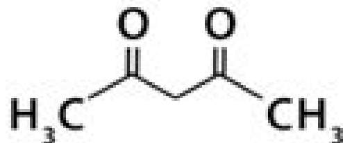
Acetylacetone
