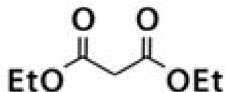
Diethyl malonate
