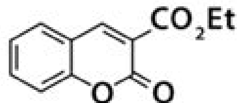
Ethyl coumarin-3-carboxylate
