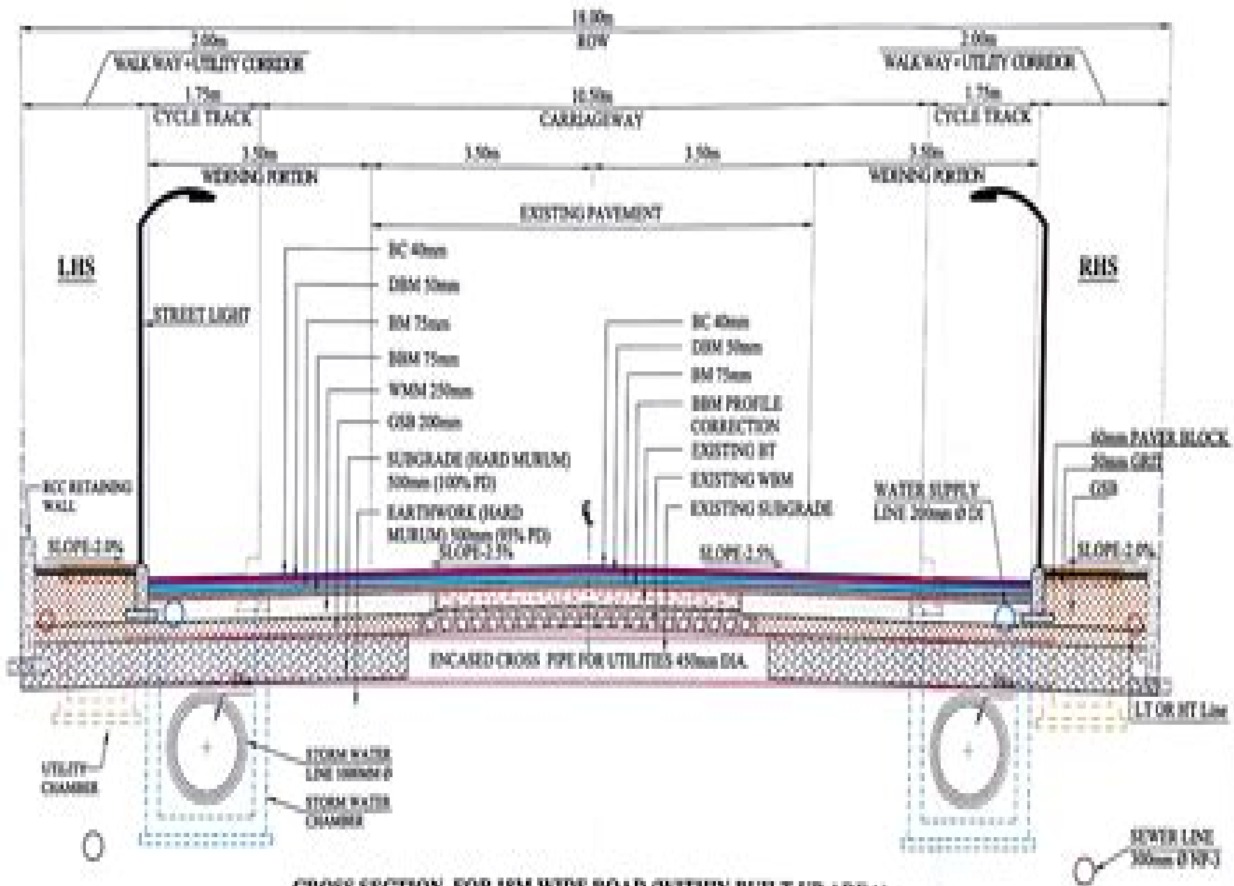
CROSS SECTION FOR 18M WIDE ROAD (WITHIN BUILT UP AREA)
