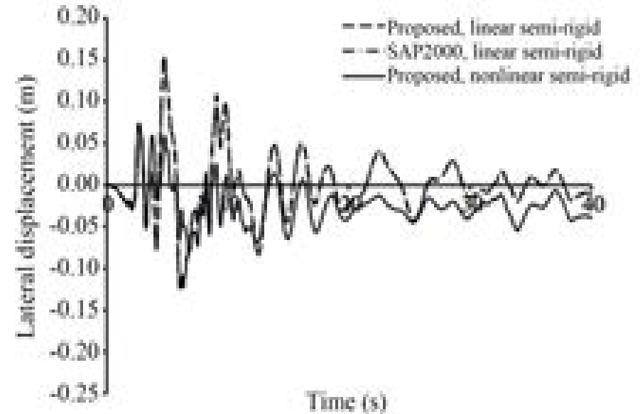
(ii) Second-order elastic responses of the semi-rigid frame
