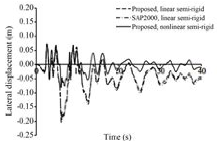
(iv) Second-order inelastic responses of the semi-rigid frame
