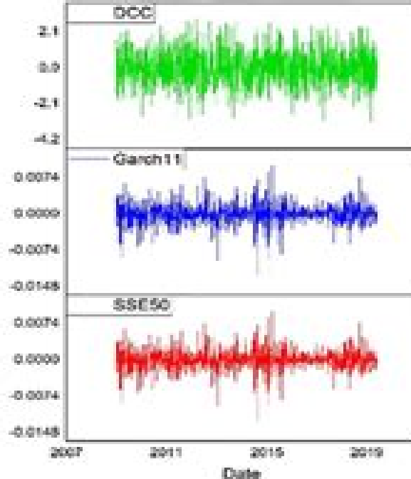
SSE50 Volatility Capturing
