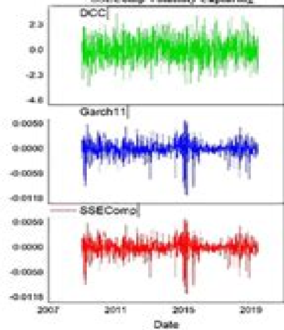
SSEComp Volatility Capturing
