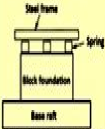
(b) Spring mounted block foundation
