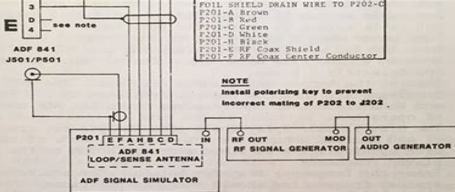
FIGURE 2-1 BENCH TEST SET-UP AND CABLE WIRING
