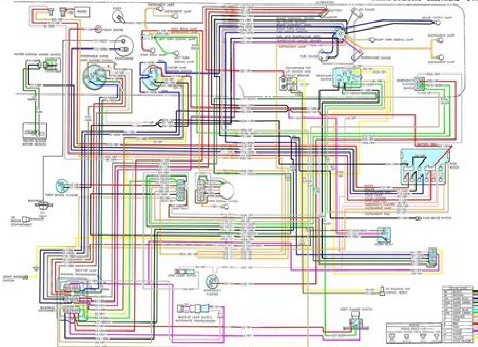
Fig. 7-Instrument Panel Wiring Diagram—Barnesville Model
