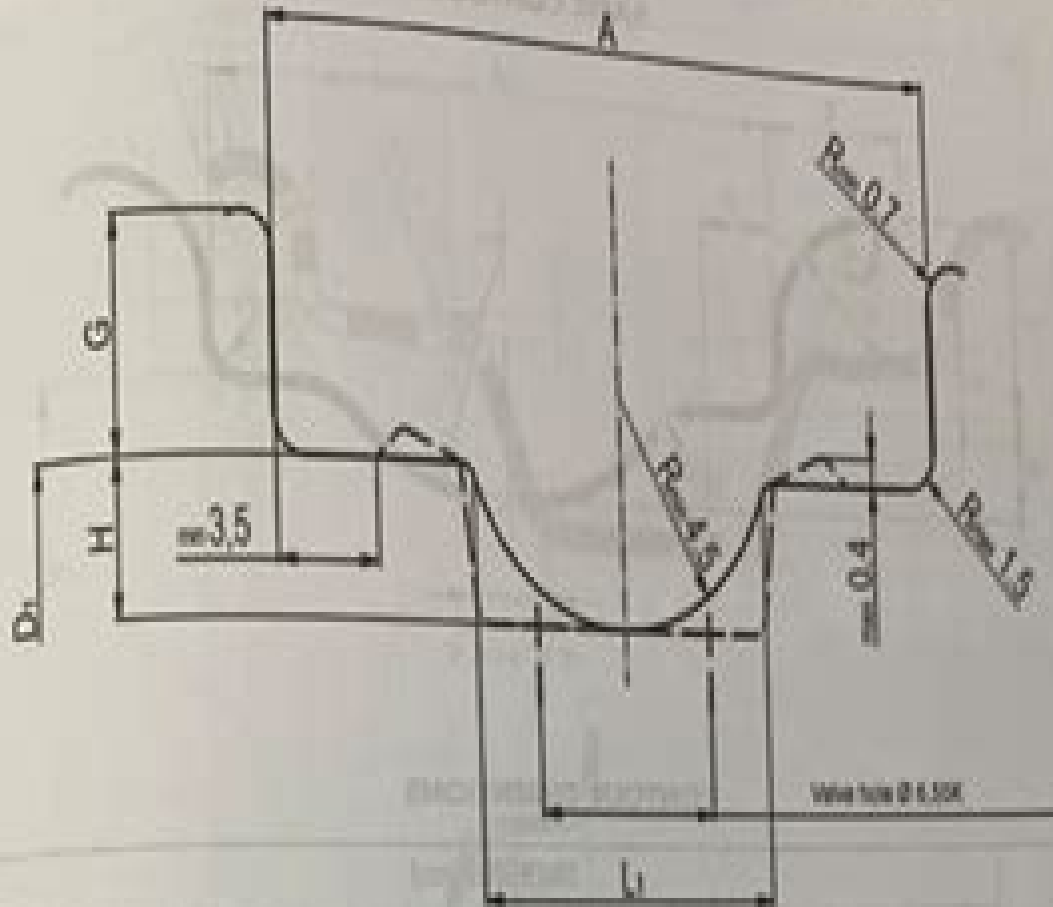
BASIC CONTOUR
