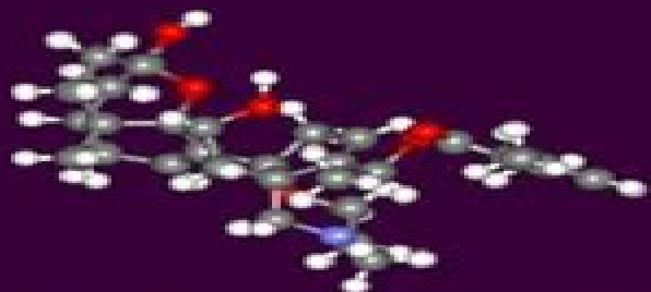
Ball-and-stick model
