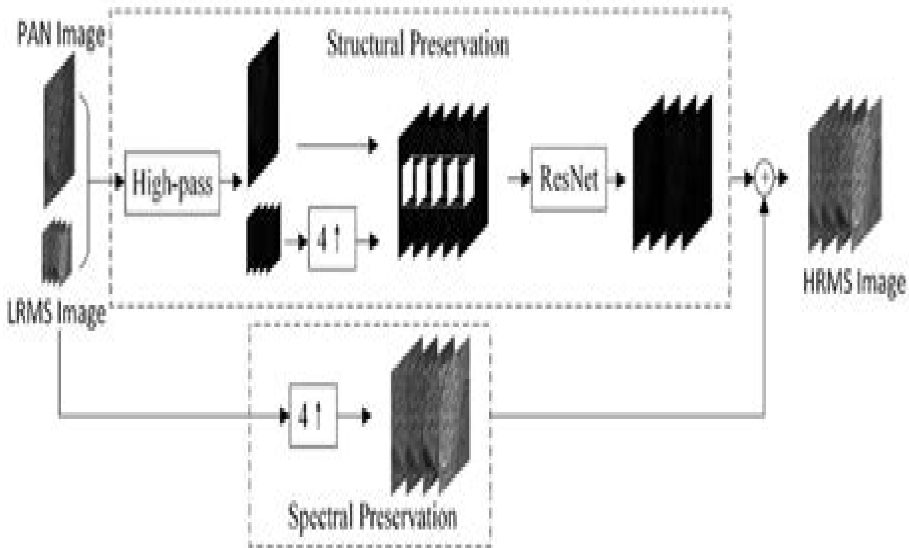
Figure 2. The deep neural network structure of the proposed pan-sharpening framework called PanNet.
