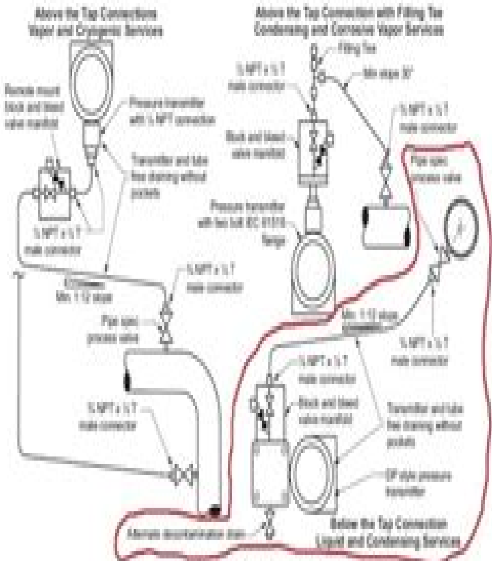
Figure 45—Pressure Transmitter Installations
