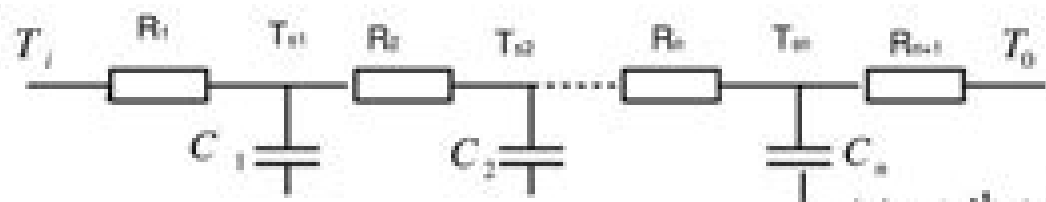
(c) n-th order lumped model
