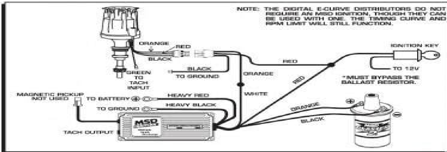
Figure 7 Connecting an MSD Ignition Control to the Digital E-Curve Distributor.
