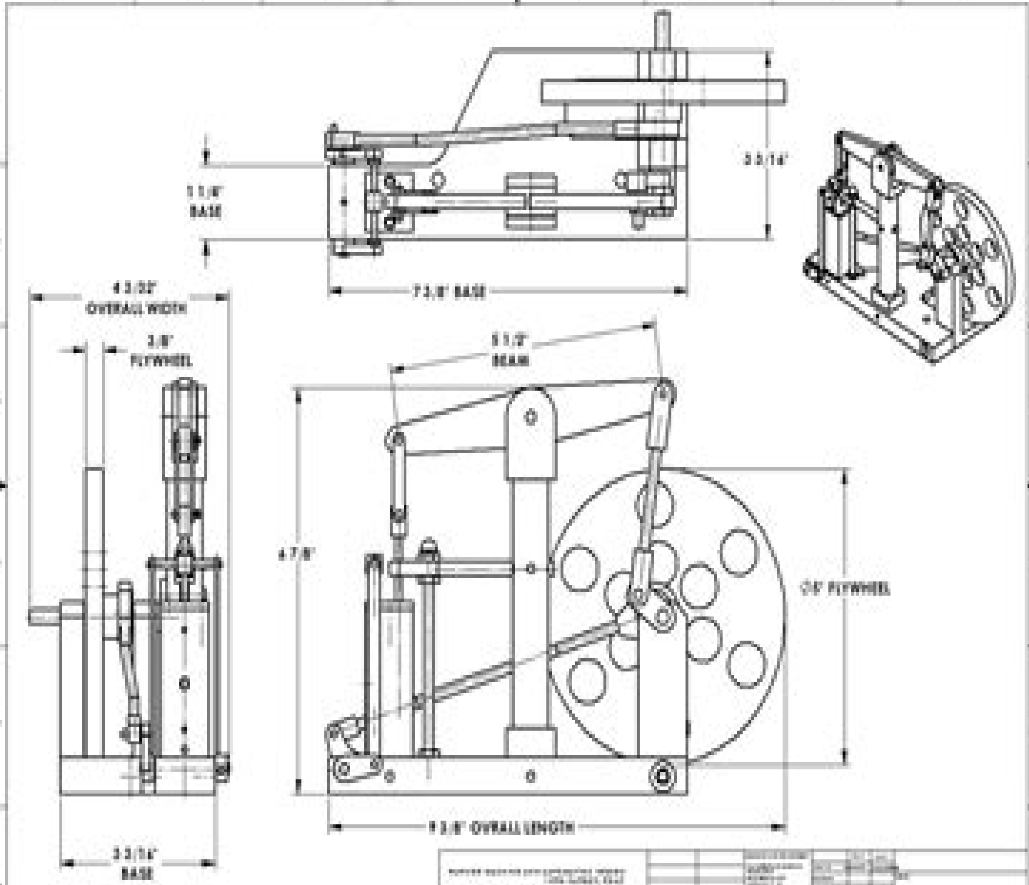
FIG. 6. A COMPLETE FIRST DRAWING SEE SECTION INSTRUCTIONS FOR PART LIST AND AUXILIARY VIEWS
