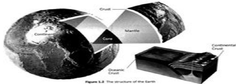
Figure 1.2 The structure of the Earth
