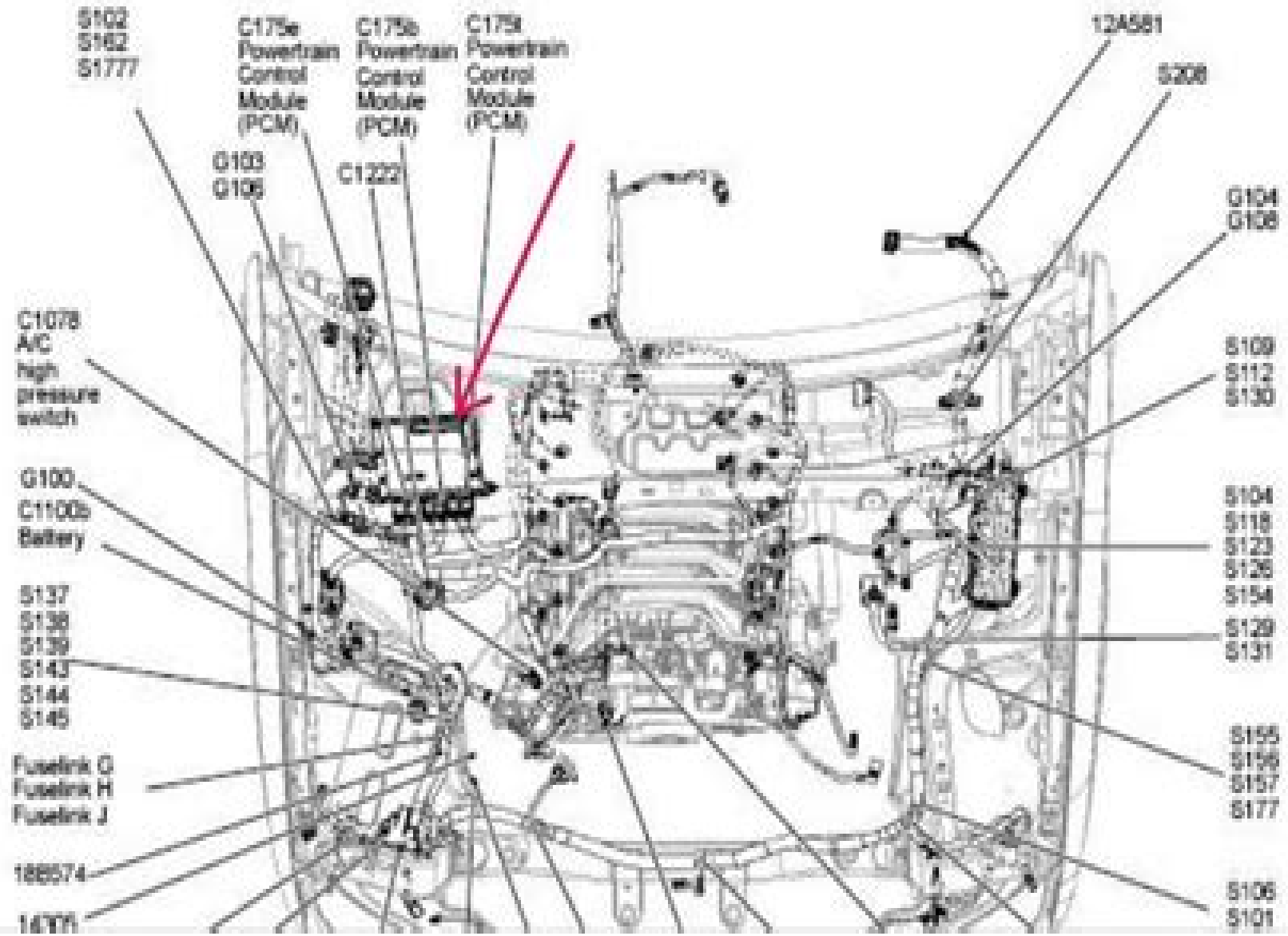
2008 Ford Pickup F350 Super Duty Fig. 2: Engine Compartment (Gas) Courtesy of FORD MOTOR CO.
