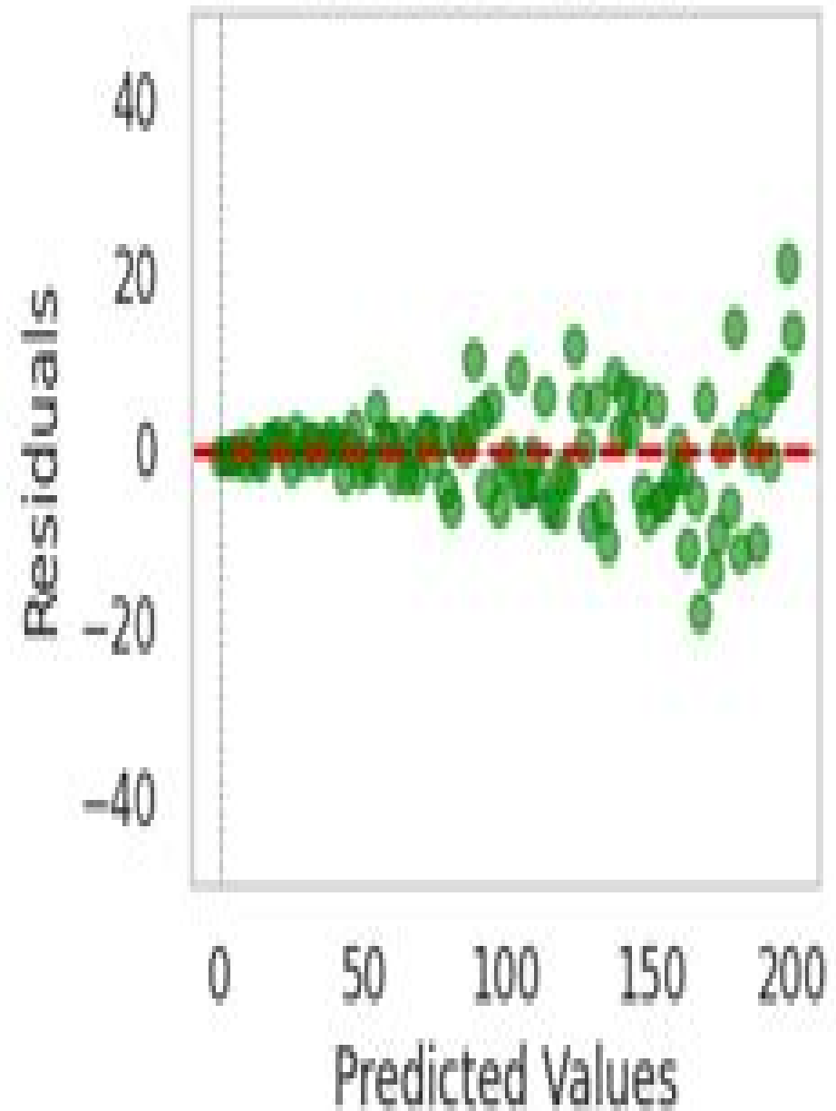
Heteroscedasticity
