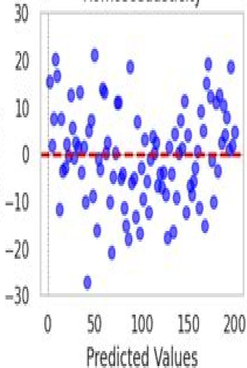
Homoscedasticity
