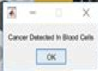
Pre-processing
