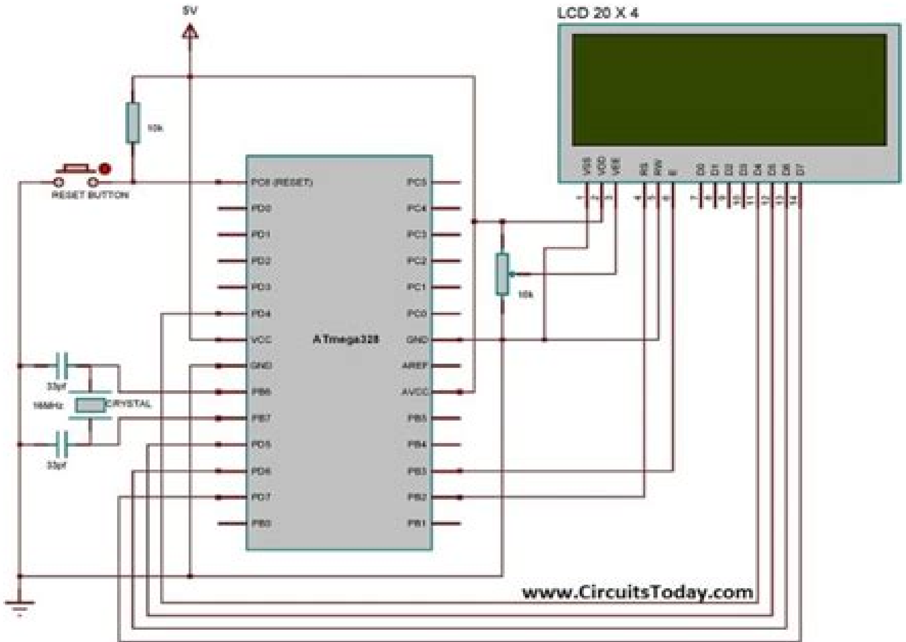
INTERFACING LCD MODULE WITH AVR IN 4-BIT MODE
