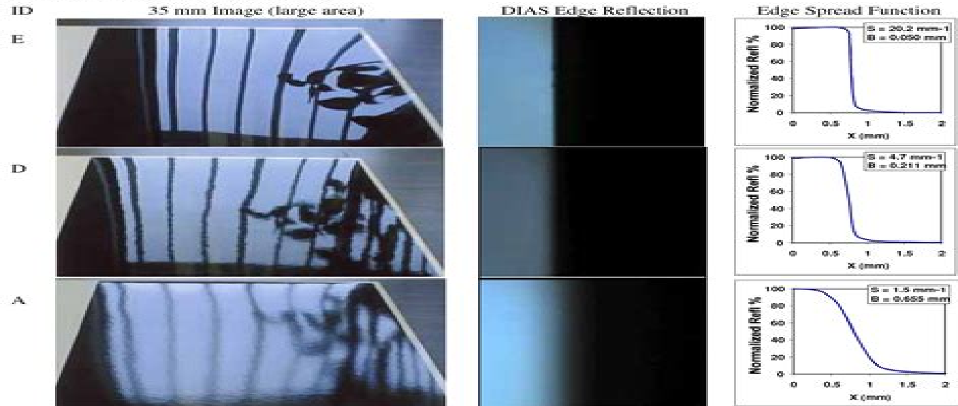
Figure 3. Correlating visual ranking (35 mm images) with instrumental DOI assessments (DIAS).
