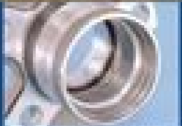
① Phenomenon: Rust Generated on Grooves at Intervals on Groove, Flank ② Cause: Moisture Contamination during Operation
