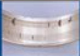
① Phenomenon: Rust Generated on Grooves at Intervals on Groove, Flank ② Cause: Bearings left (unused) for Long Period under Moist Conditions
