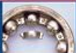
① Phenomenon: Flaking on Grooves, Spalls, Grooves, Ring Ribs ② Cause: Excessive Load due to Misalignment
