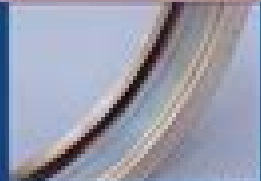
① Phenomenon: Flaking on Grooves, Spalls, Surface of Grooves ② Cause: Inadequate Lubrication Method, or Inappropriate Lubricant
