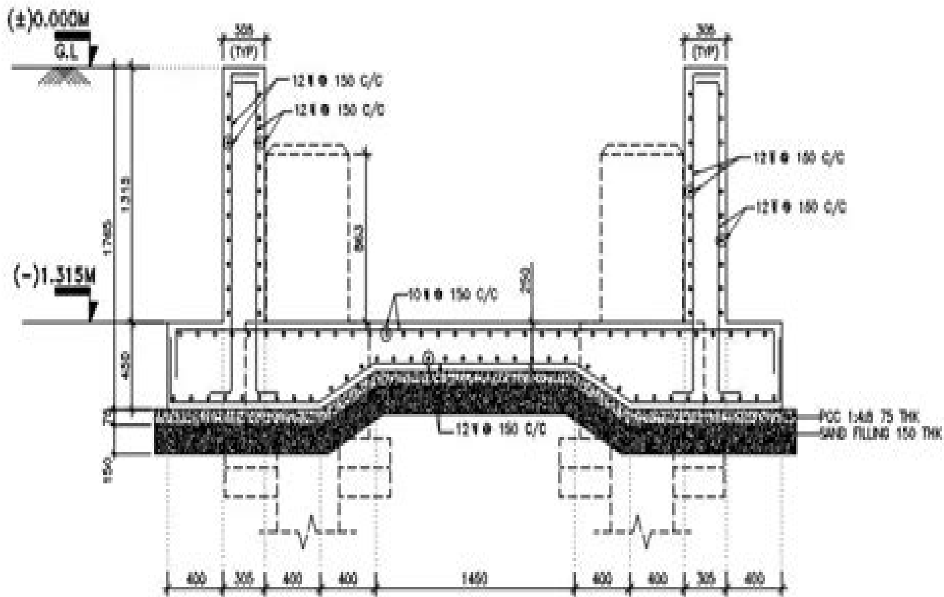
SECTION 4-4
