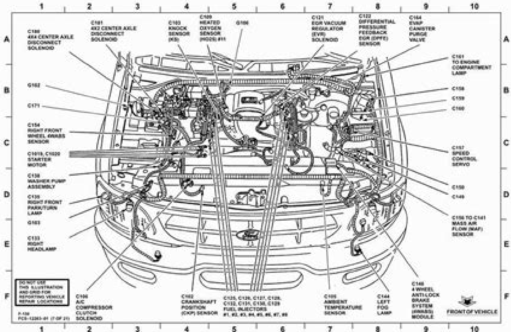
5.4L ENGINE (2 OF 2) (NGV SIMILAR)
