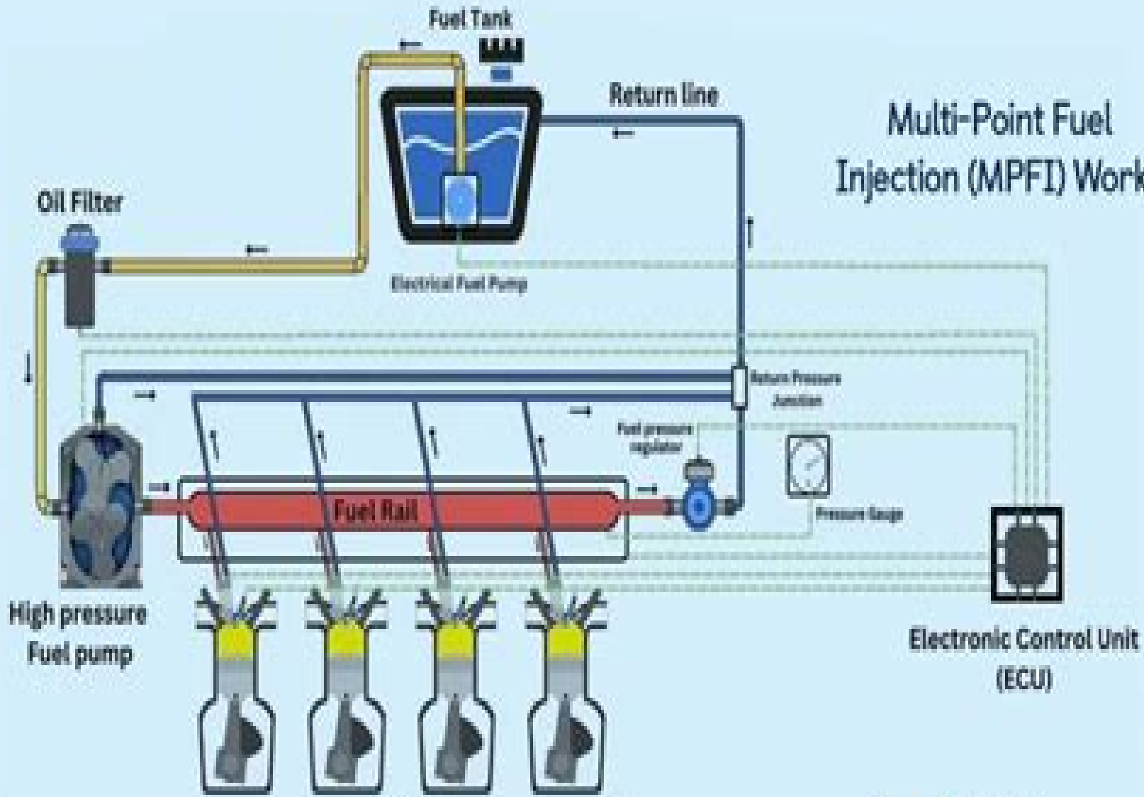
Multi Point Fuel injection system
