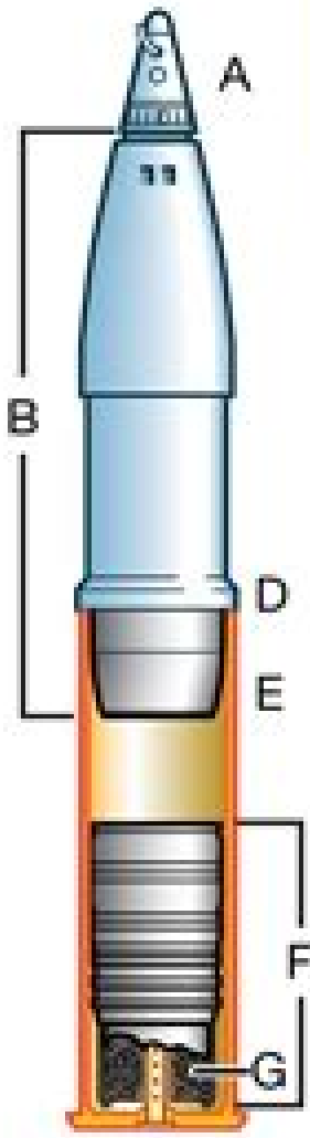
semifixed ammunition
