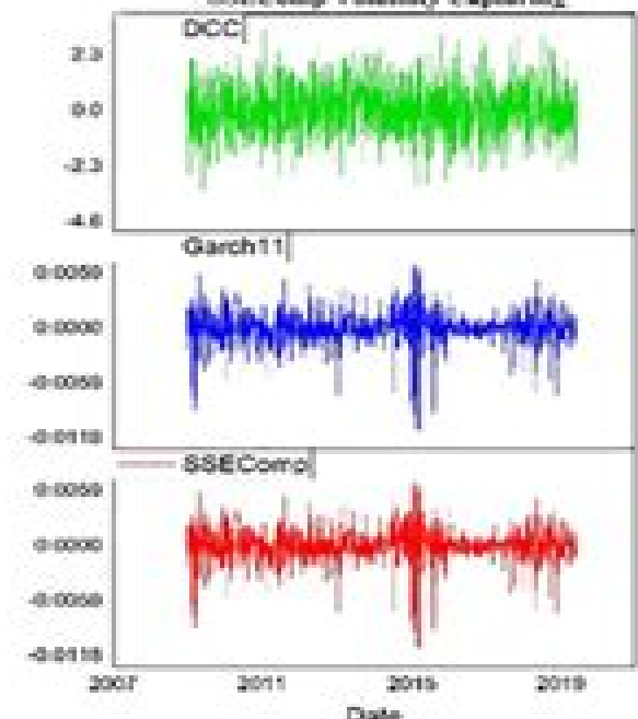
SSEComp Volatility Capturing
