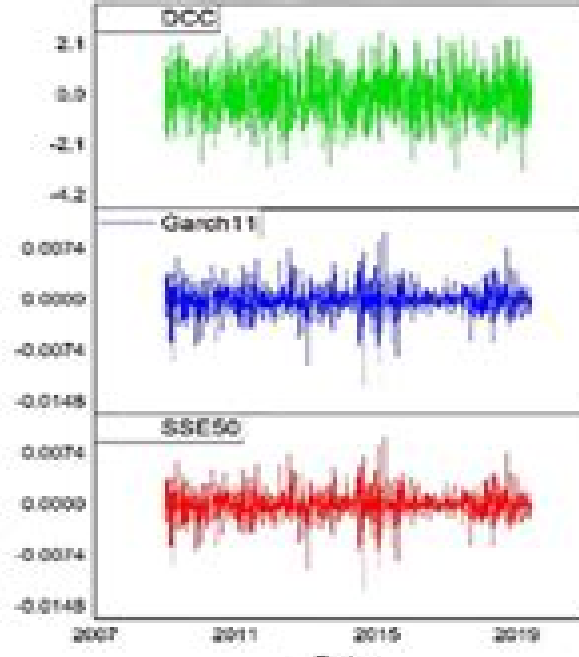
SSE50 Volatility Capturing
