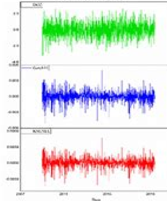
SSEComp Volatility Capturing
