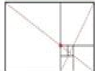
The Golden Section Point
