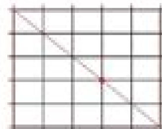
The Golden Section Point of a Rectangle
