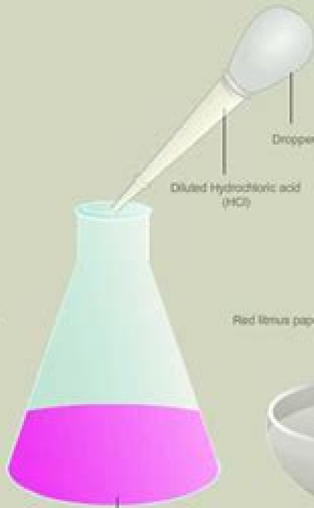
Sodiumhydroxide + Phenolphthalein
