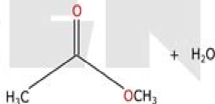
Methyl ethanoate
