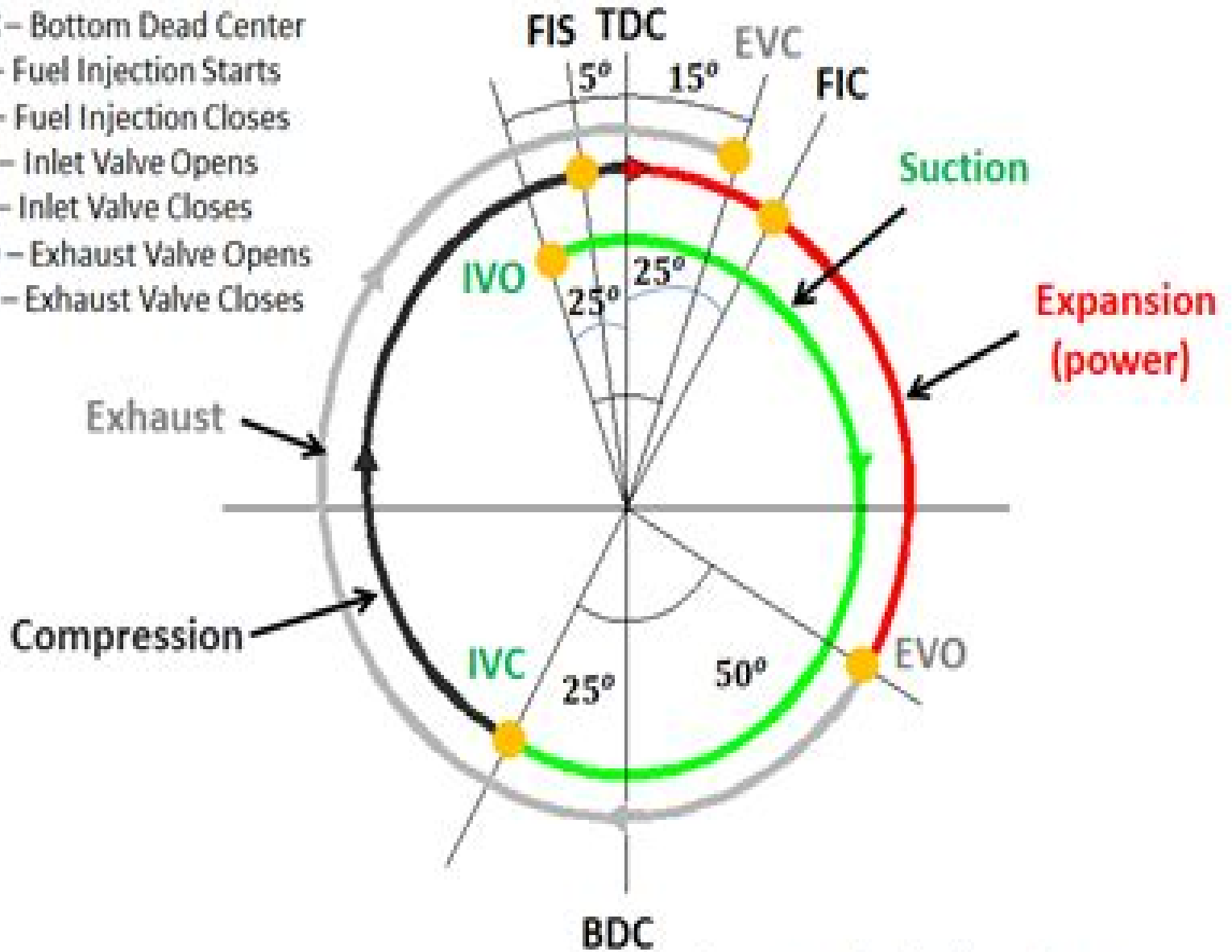
Valve Timing Diagram of 4 Stroke Diesel Engine
