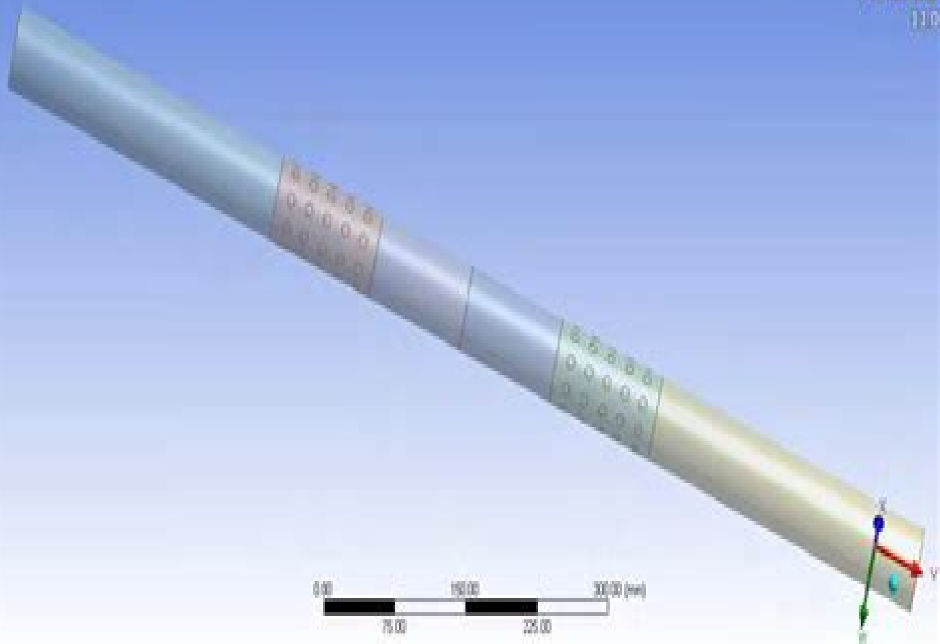
Fig. 3. Model of the shaft with sleeves and the dimensions of the shaft.
