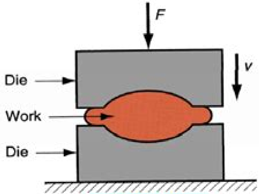
Forging
